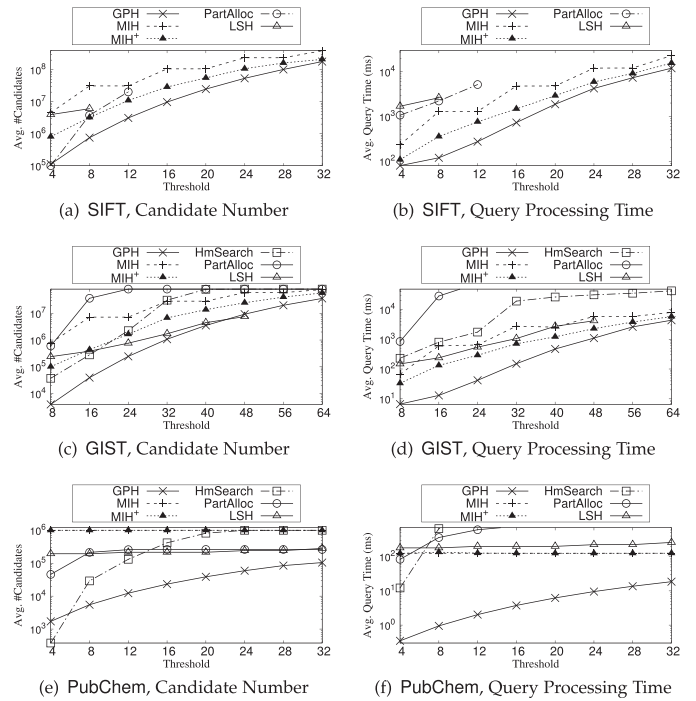
Fig. 7. Comparison with alternatives - candidate number &amp; time.
