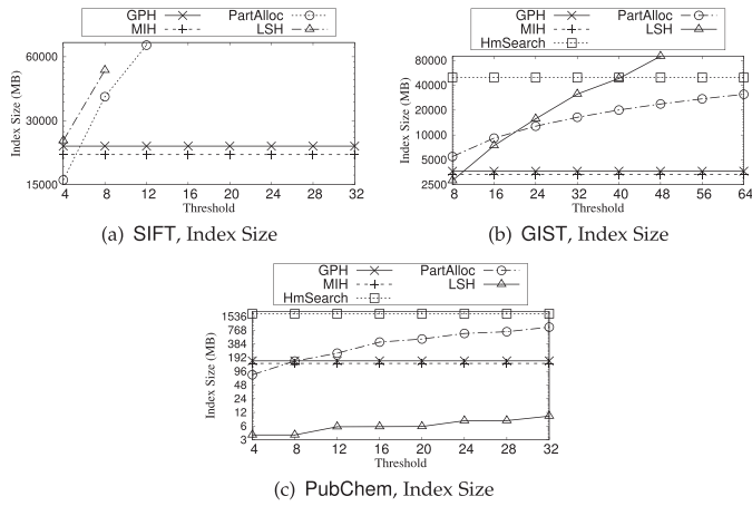
Fig. 6. Comparison with alternatives - index size.
