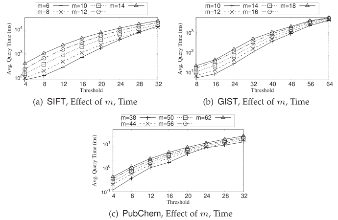
Fig. 5. Effect of partition size.
