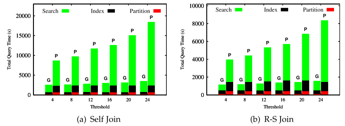
Fig. 9. Join time breakdown.
