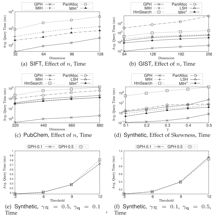
Fig. 8. Varying number of dimensions and skewness.
